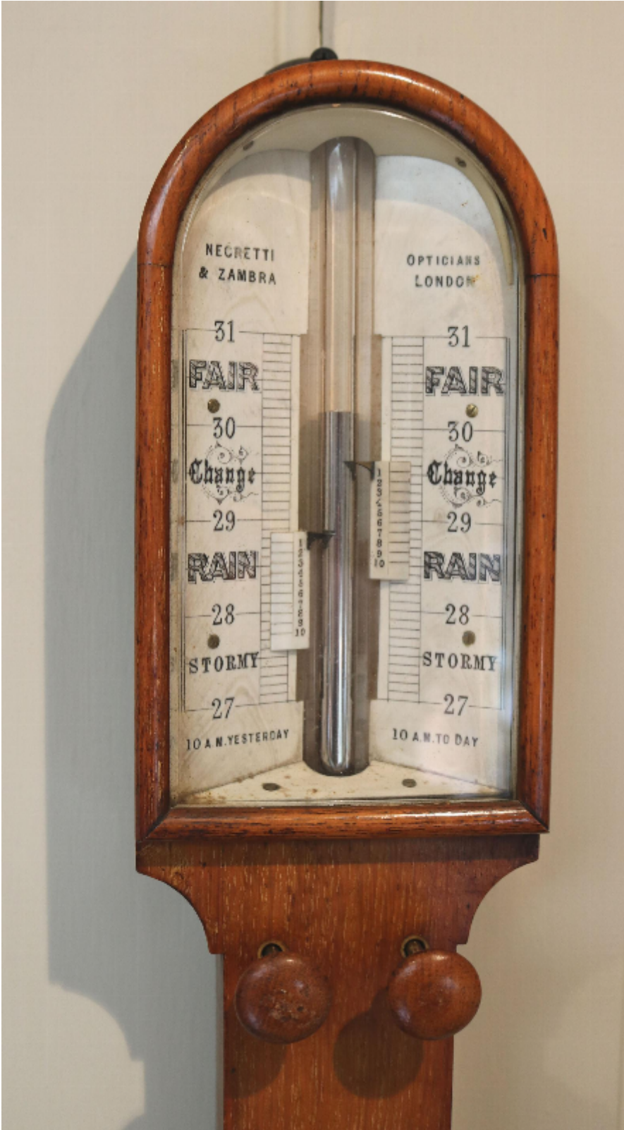
Solid Oak Stick Barometer NEGRETTI & ZAMBRA
